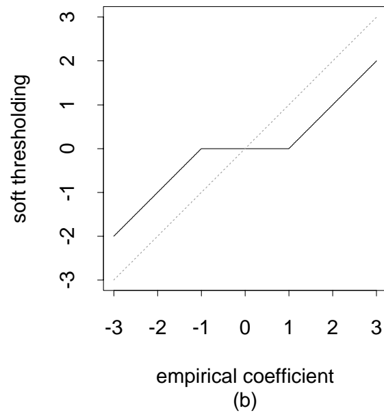
Figure 4: (a) The hard thresholding rule for \lambda = 1 ; (b) The soft thresholding rule for \lambda = 1 .
