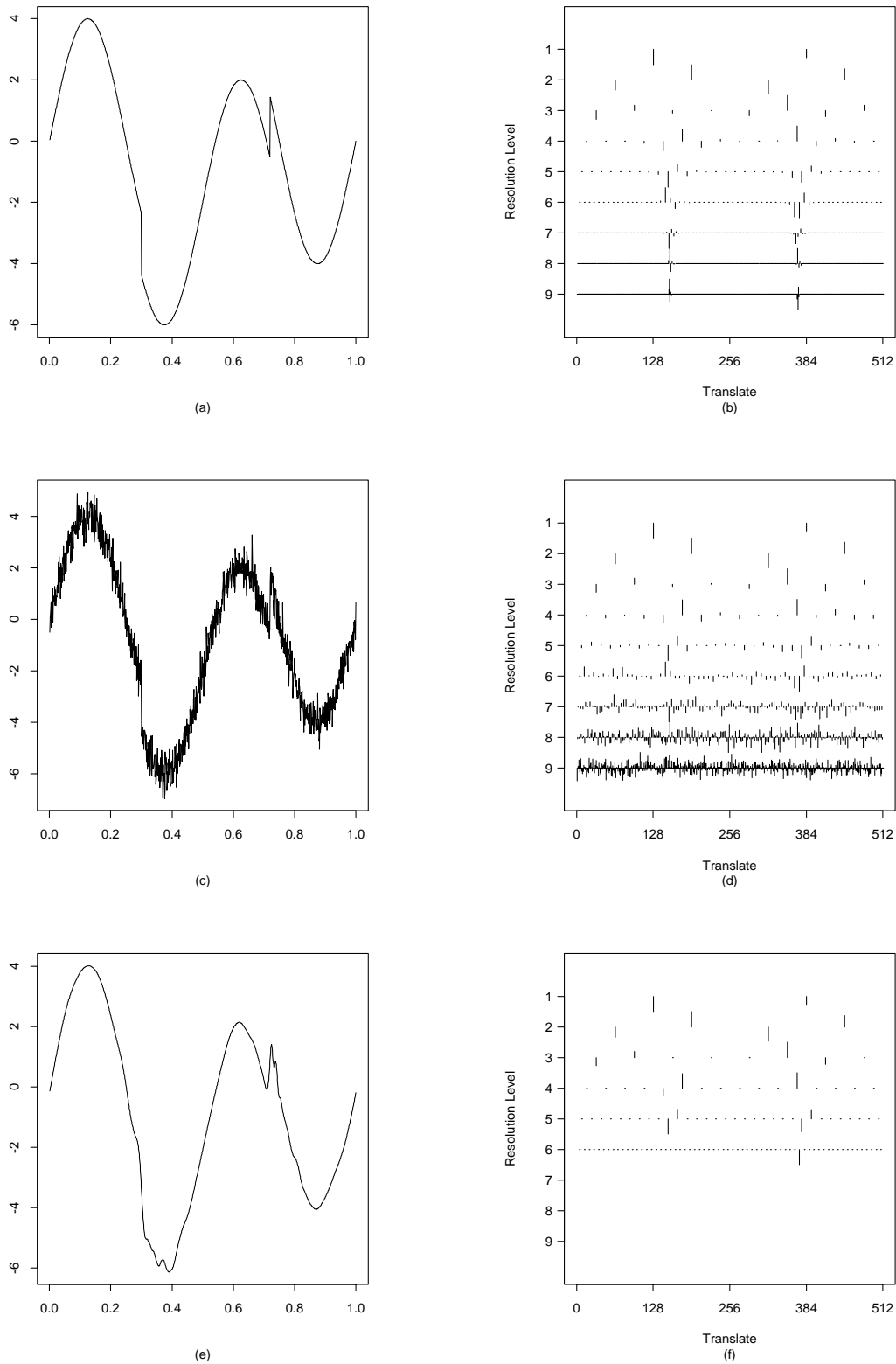
Figure 5: (a) The 'Heavisine' function sampled at 1024 data points uniformly spaced on [0, 1] ; (b) The wavelet decomposition of (a) using the Extremal Phase wavelet with six vanishing moments; (c) The 'Heavisine' function corrupted with independent random noise N(0, \sigma^2) (root signal-to-noise ratio is 7); (d) The wavelet decomposition of (c) using the Extremal Phase wavelet with six vanishing moments; (e) The reconstruction of the 'Heavisine' function based on (f) the the universal threshold applied to (d).
